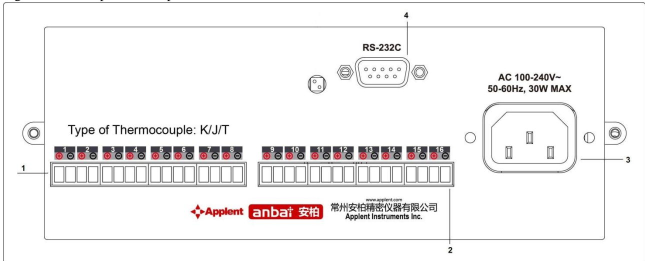
Figure 3-2 Back panel description
