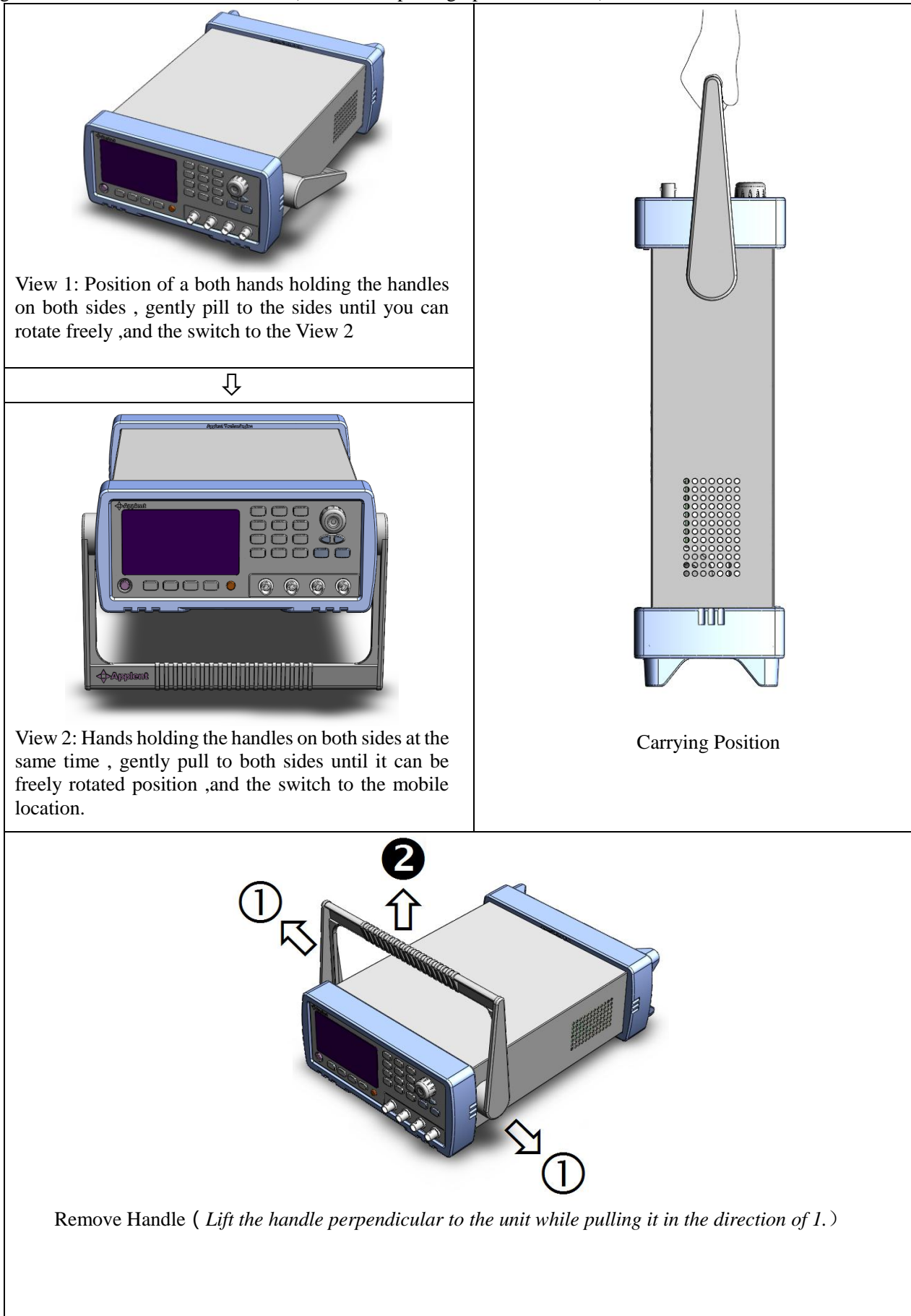
Figure 1-1 The instrument handle (schematics, panel graphics and is not)
